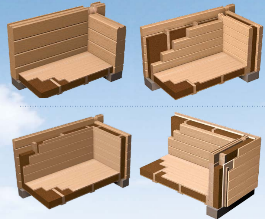
Thermo wall inside
